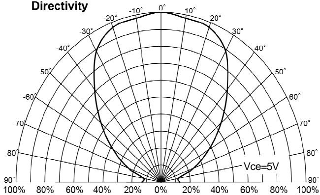
Directivity
