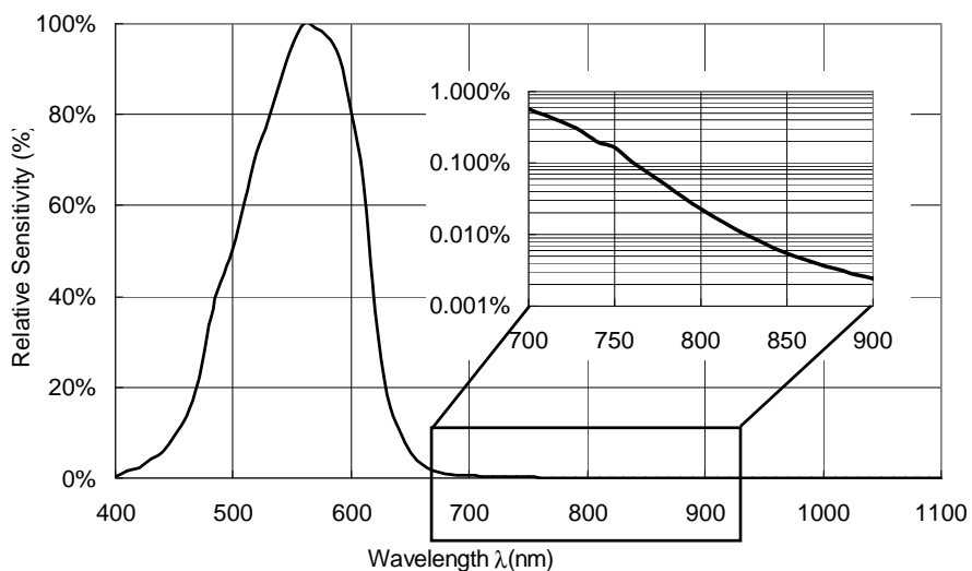
Spectral Response
